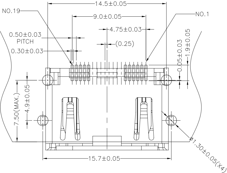
RECOMMENDED PCB LAYOUT (THICKNESS=1.6±0.15mm)
