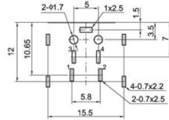
PCB LAYOUT (VIEWED FROM COPPER SIDE)
