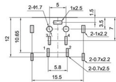
PC B LAYOUT (VIEWED FROM COPPER SIDE)
