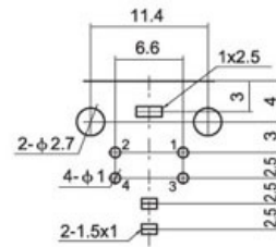
PC.B LAYOUT (VIEWED FROM COPPER SIDE)
