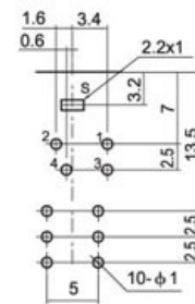
PC.B LAYOUT (VIEWED FROM COPPER SIDE)
