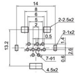
P.C.B LAYOUT (VIEWED FROM COPPER SIDE)
