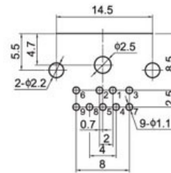
PC.B LAYOUT (VIEWED FROM COPPER SIDE)
