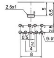
PC B LAYOUT (VIEWED FROM COPPER SIDE)
