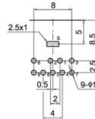
PC B LAYOUT (VIEWED FROM COPPER SIDE)
