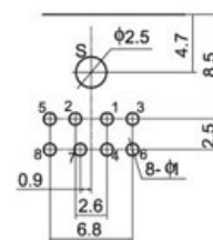
PCB LAYOUT (VIEWED FROM COPPER SIDE)
