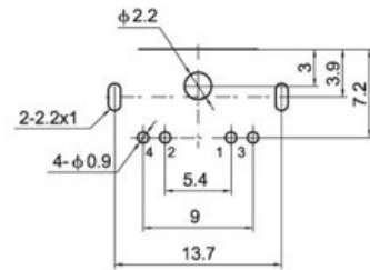
PC.B LAYOUT (VIEWED FROM COPPER SIDE)
