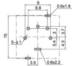
P.C.B LAYOUT (VIEWED FROM COPPER SIDE)
