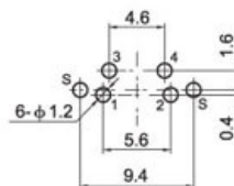
PC.B LAYOUT (VIEWED FROM COPPER SIDE)
