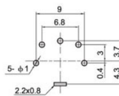
PCB LAYOUT (VIEWED FROM COPPER SIDE)
