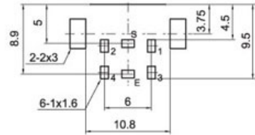
PC B LAYOUT (VIEWED FROM COPPER SIDE)
