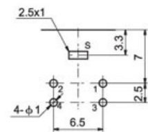
PC.B LAYOUT (VIEWED FROM COPPER SIDE)
