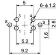
P.C.B LAYOUT (VIEWED FROM COPPER SIDE)
