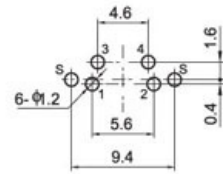
P.C.B LAYOUT (VIEWED FROM COPPER SIDE)
