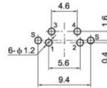
PC.B LAYOUT (VIEWED FROM COPPER SIDE)
