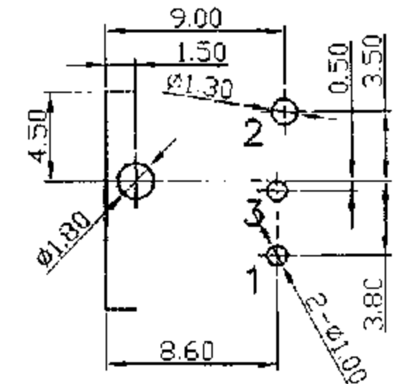
Pin Hole Layout (Jack Bottom View)
