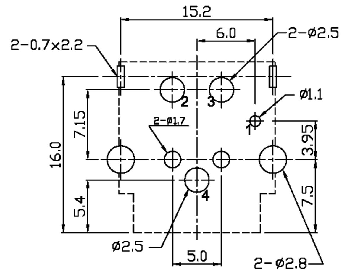
P.C.B. LAYOUT(±0.1) (BOTTOM VIEW)
