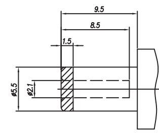
Mating Plug
