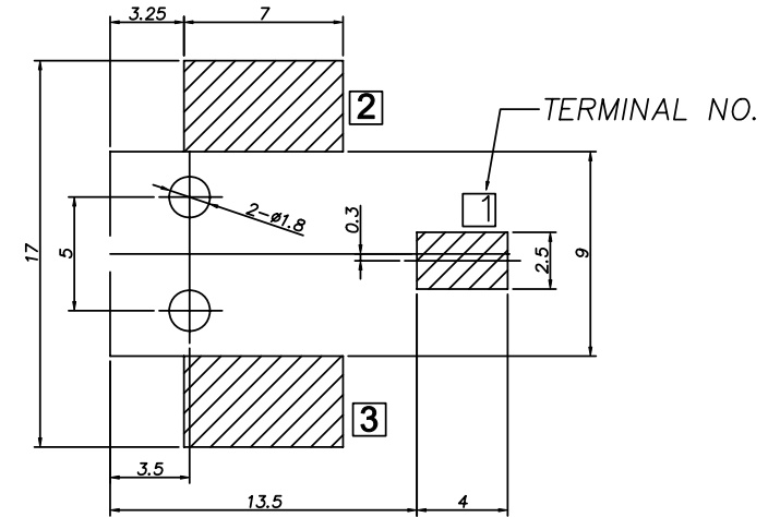
P. C. B Layout (Printed-sided view)
