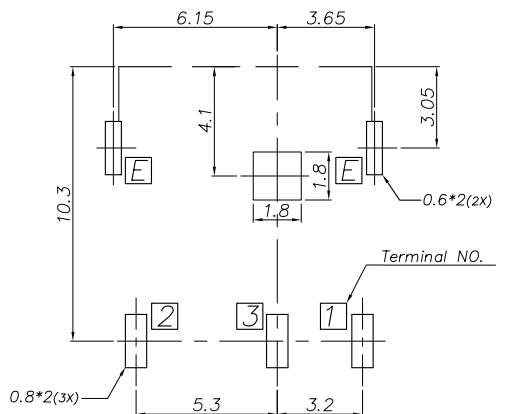
RECOMMENDED P.C.B. LAYOUT UNSPECIFIED TOLERANCE: ±0.05 (BOTTOM VIEW)
