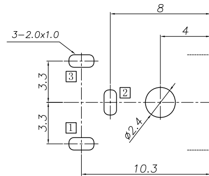
RECOMMENDED P. C. B. LAYOUT UNSPECIFIED TOLERANCE: ±0.1 (Copper-sided view)
