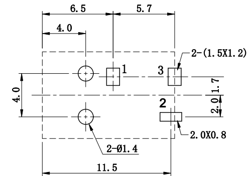
RECOMMENDED P.C.B LAYOUT TOP VIEW, TOLERANCES:±0.05mm
