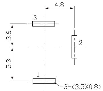
P.C.B TOP LAYOUT VIEW
