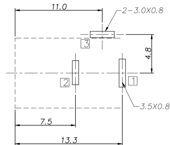
P. C. B Layout (Printed-sided view)
