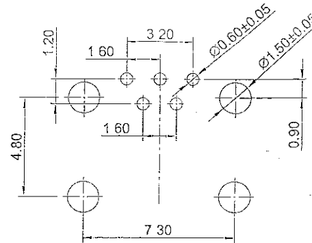
PC BOARD LAYOUT ±0.10mm
