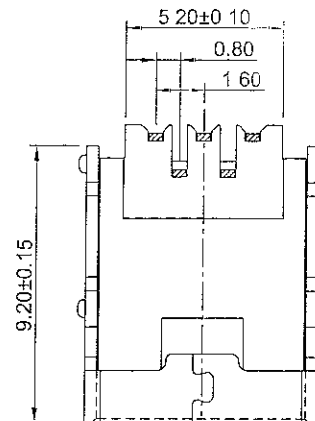
PC BOARD LAYOUT ±0.10mm
