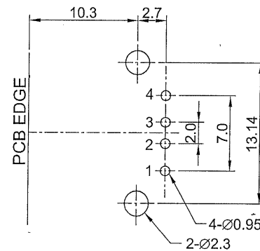
PCB LAYOUT±0.1mm (BOTTOM VIEW)
