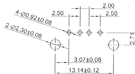
PC BOARD LAYOUT ±0.1mm
