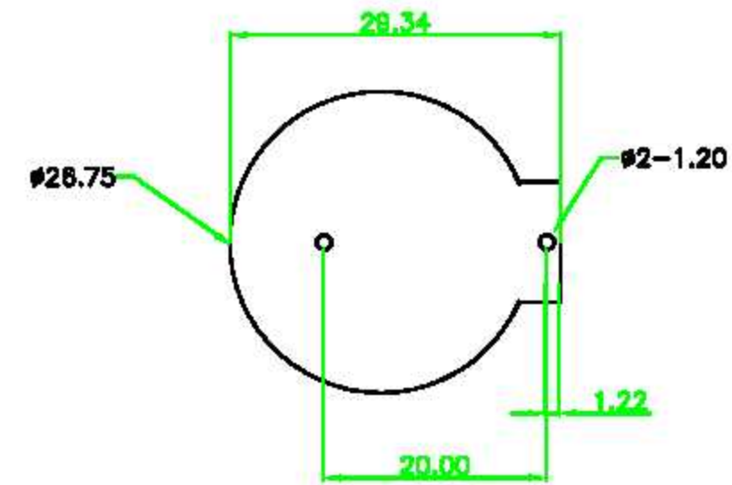
PCB HOLE LAYOUT
