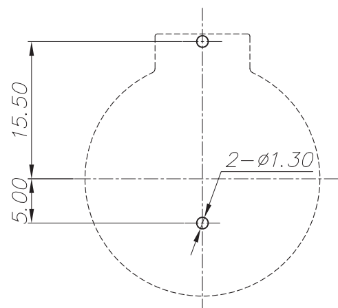
PCB Holes Diagram Top View
