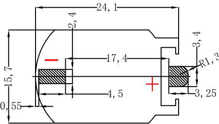
PCB Layout Diagram Top View
