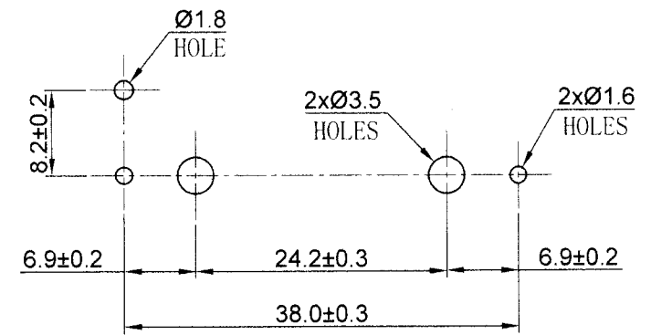
PCB/MOUNTING LAYOUT
